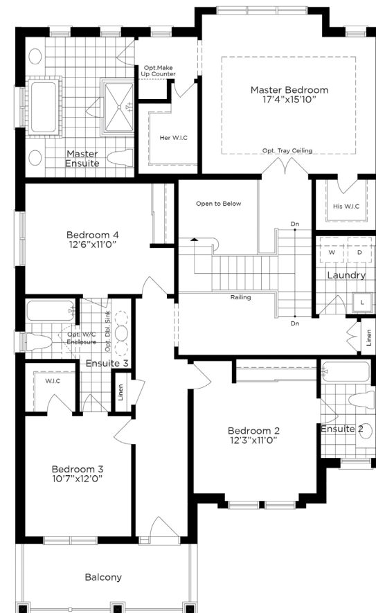
Second Floor
