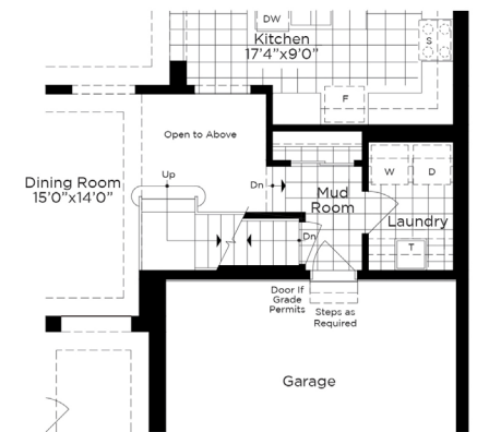
First Floor 5 Bedroom Layout W/Laundry Relocated Elevation B & R
